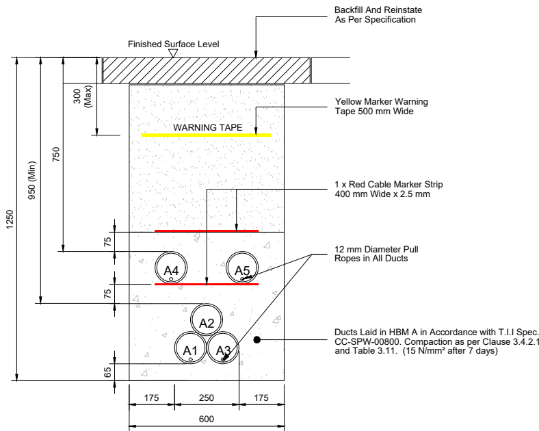
A=125 mm: Outer Diameter HDPE ESB Approved Duct, SDR=17.6 All Dimensions in Millimetres.
